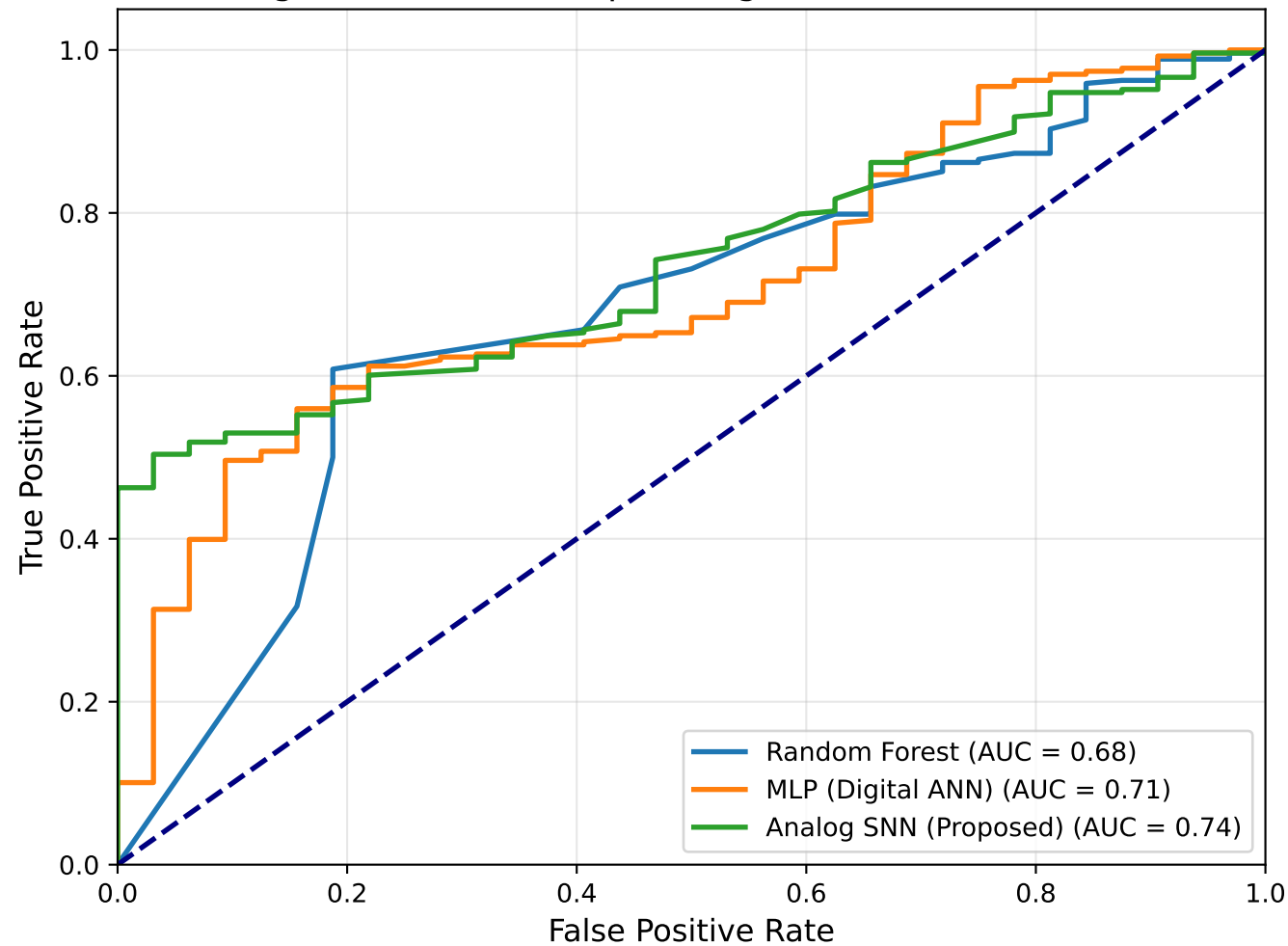
Figure 6: Receiver Operating Characteristic (ROC)
